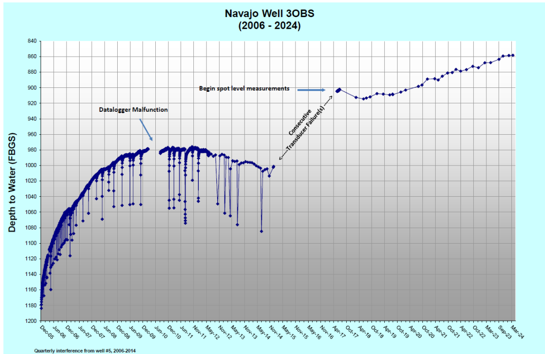
Figure 8. Observation Well NAVOBS3 Response (USGS Cooperators Meeting Handout, June 2024).
