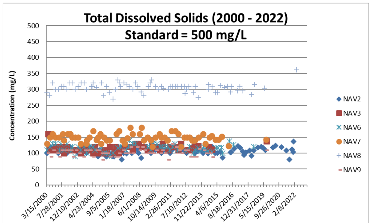
Figure 17. TDS Concentrations in PWCC N-aquifer Wells (2000 – 2022) (PWCC, 2023).
