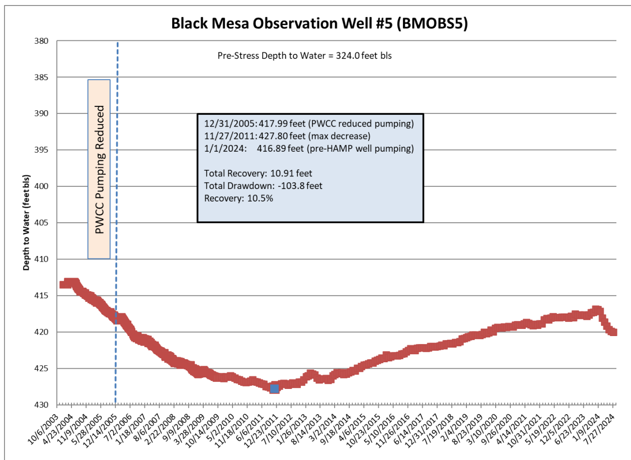
Figure 7. Black Mesa Observation Well BM-5 Water Level Measurements (USGS, 2024).
