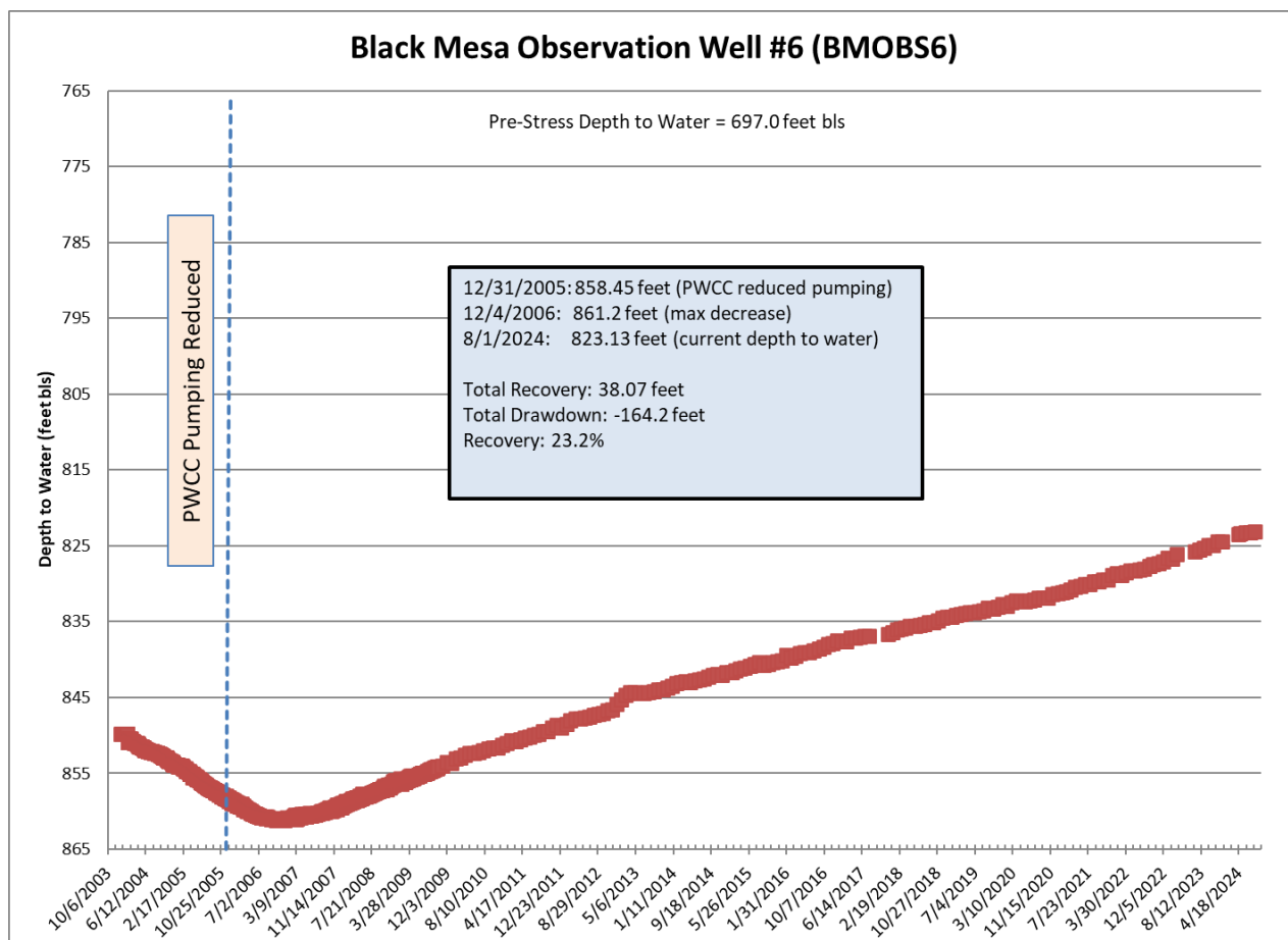
Figure 6. Black Mesa Observation Well BM-6 Water Level Measurements (USGS, 2024).
