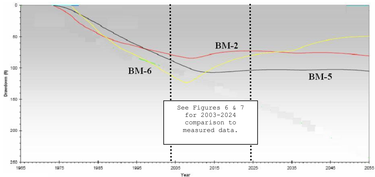
Figure 5. 3D Flow Model Simulated Water Level Response: BM-2, BM-5, BM-6 (BLM, 2017).
