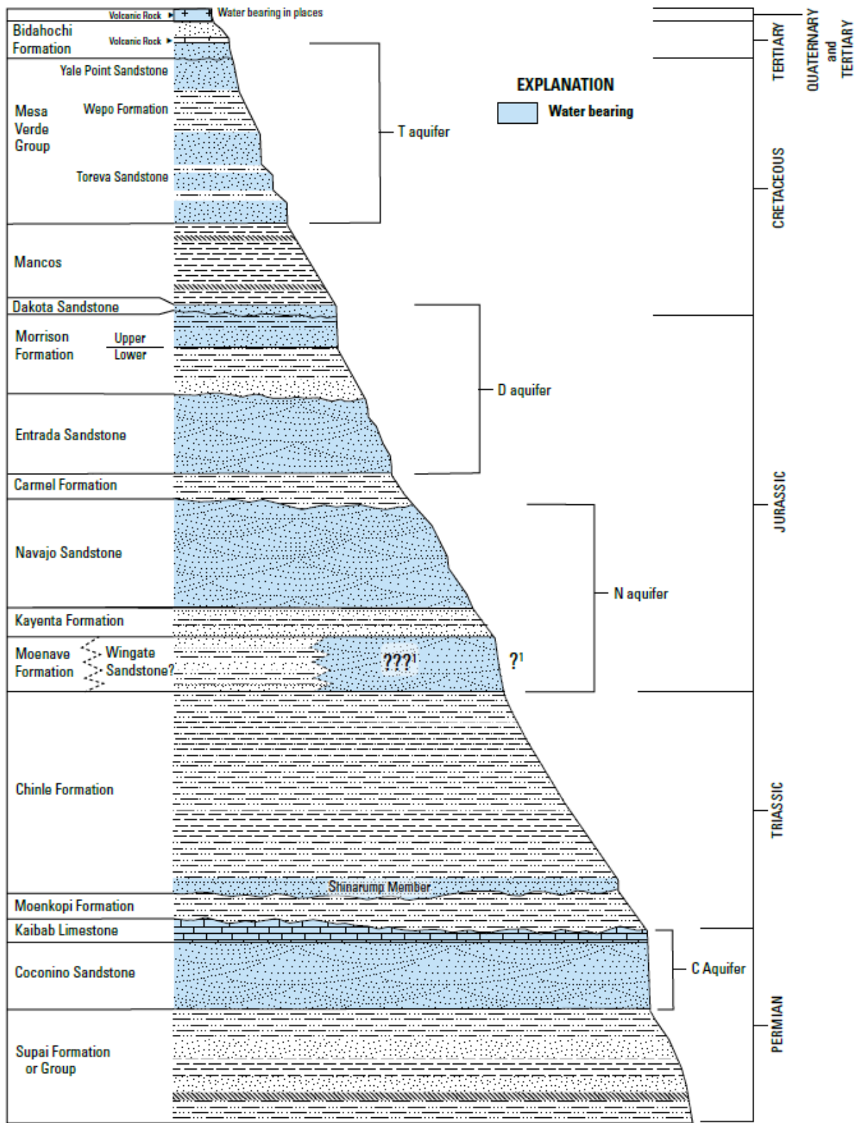
Figure 2. Rock Formations and Major Aquifer Zones of the Black Mesa Area (Mason, 2024).
