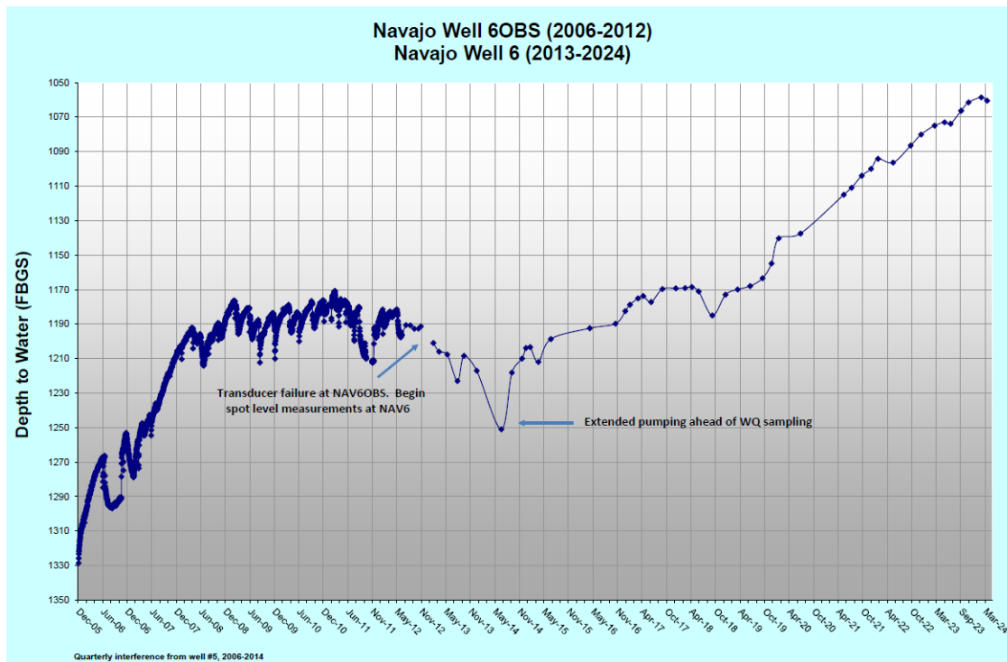
Figure 9. Observation Well NAVOBS6 Response (USGS Cooperators Meeting Handout, June 2024).
