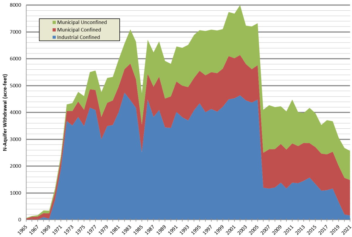
Figure 10. Historical Total N-Aquifer Withdrawal 1965 - 2021 (Mason, 2024).
