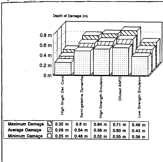
Figure 5 Zones of predicted damage
