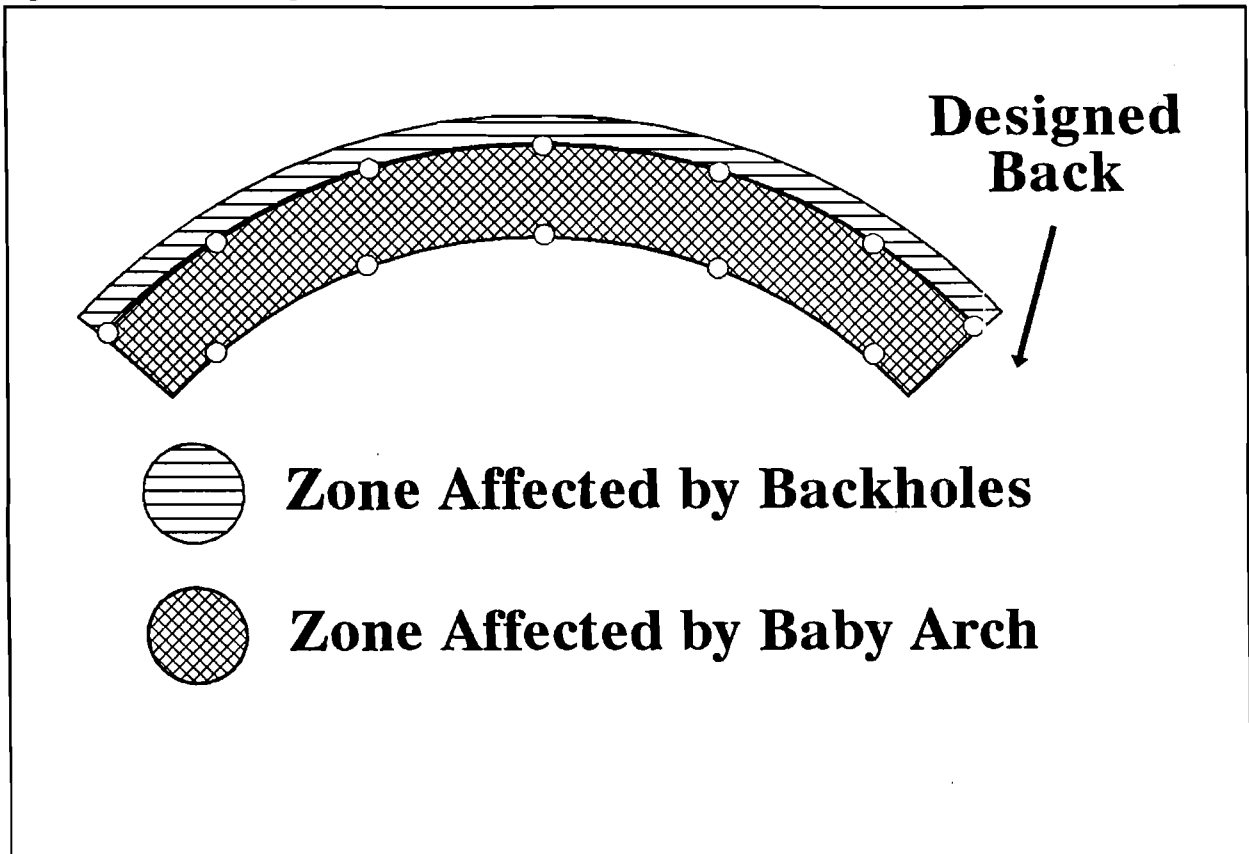
Figure 4 Damage Zones from Baby arch and Back holes.
