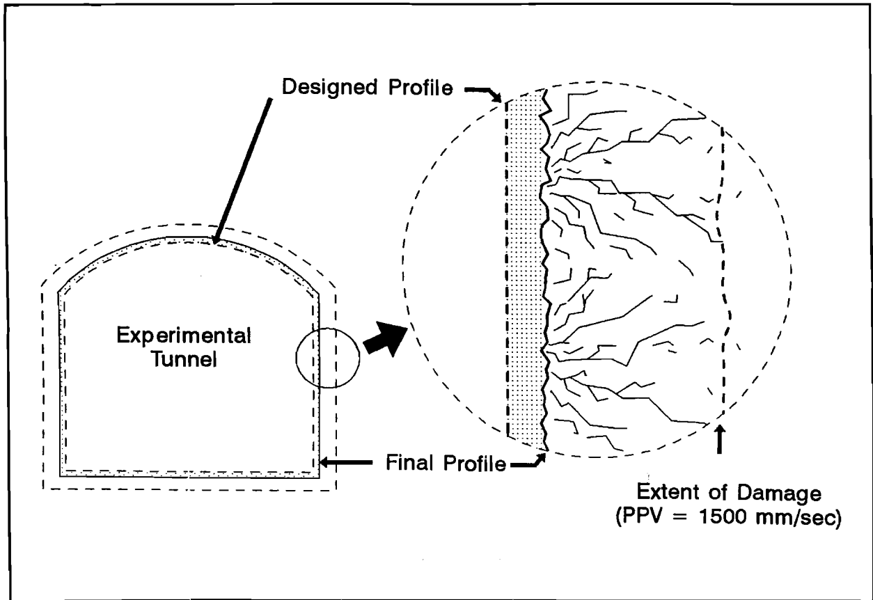
Figure 3 Profiles of the opening and extent of damage.
