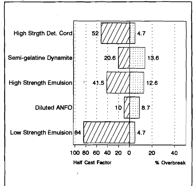
Figure 7 Half Cast Factor and Percent Overbreak.
