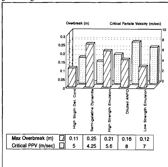
Figure 6 Critical PPV at maximum Overbreak.
