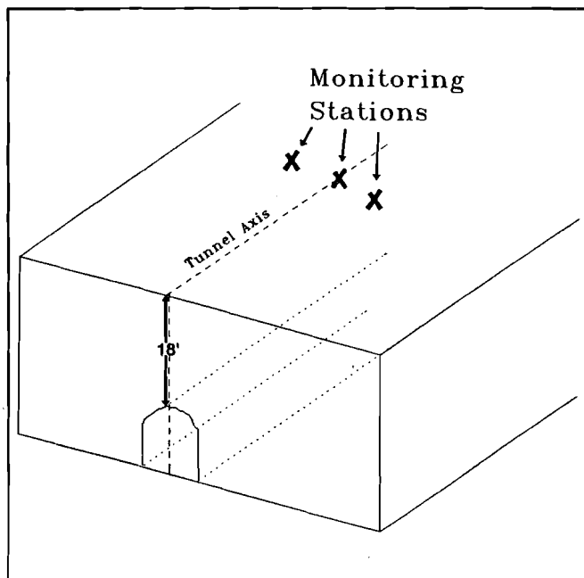
Figure 1 Location of vibration monitoring stations.
