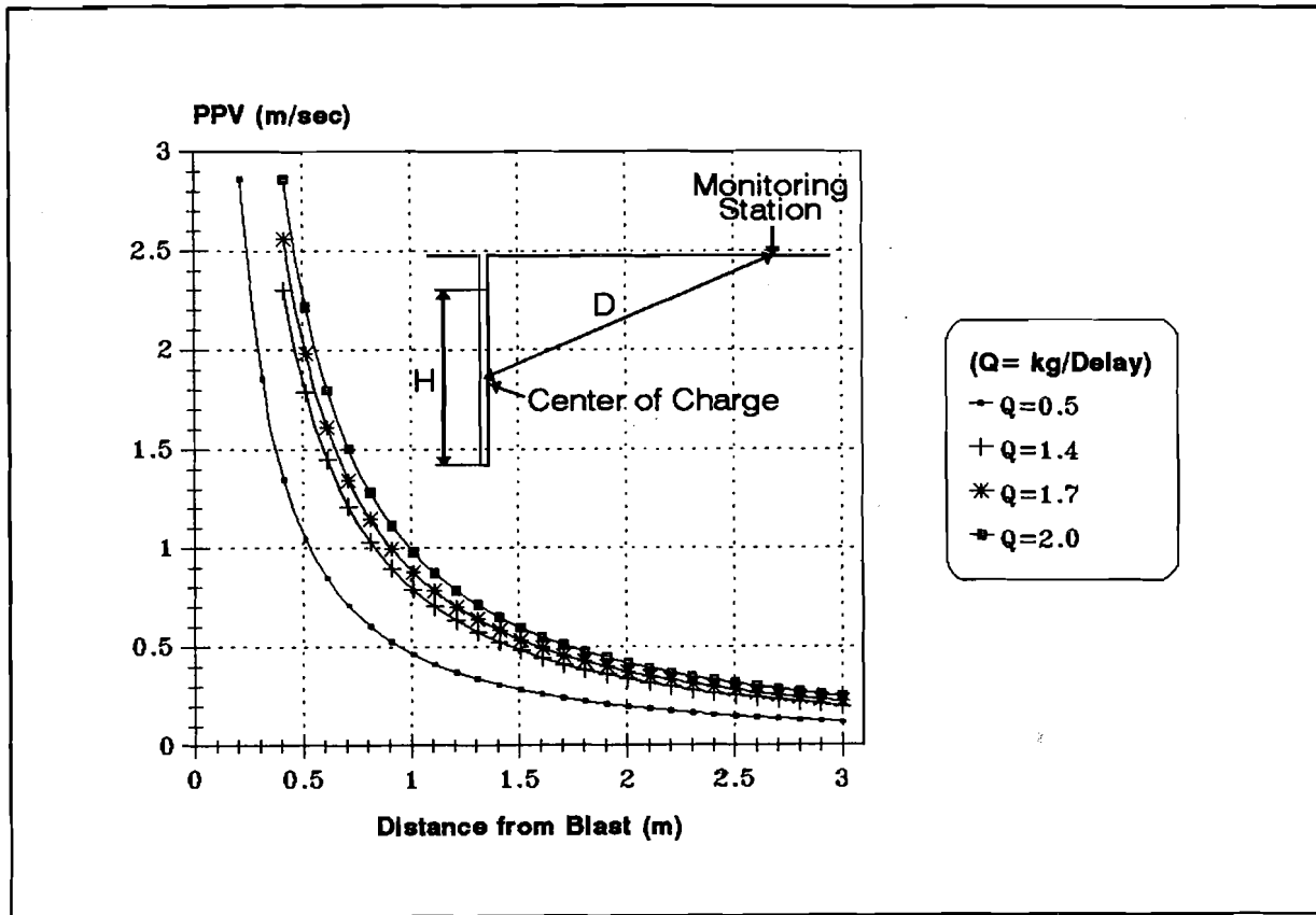
Figure 2 PPV vs Distance from blast for different charge concentrations.
