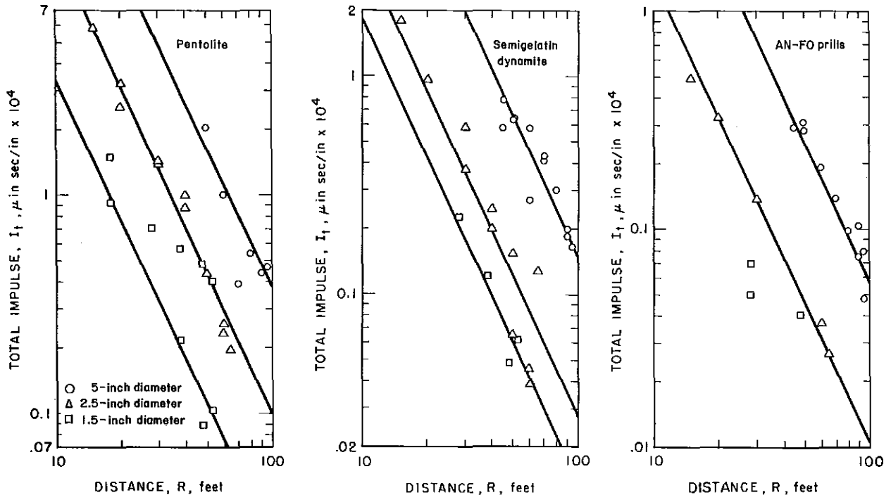
FIGURE 8. - Total Impulse Versus Distance.
