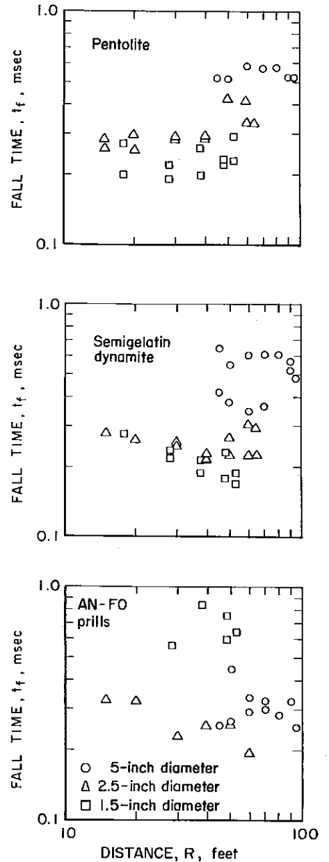
FIGURE 4. - Fall Time Versus Distance.
